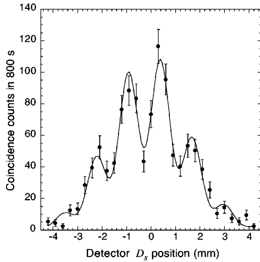
FIG. 5. Coincidence counts when QPW1, QWP2, and POL1 are in place. POL1 was set to \theta + \pi/2 , the angle of the fast axis of QWP2. Interference has been restored in the antifringe pattern.
